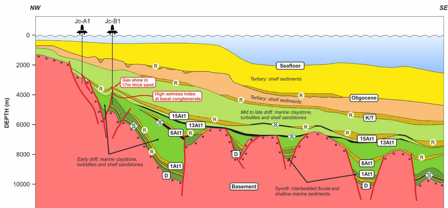
Geological cross section of the Durban Basin (courtesy of Petroleum Agency of South Africa).
