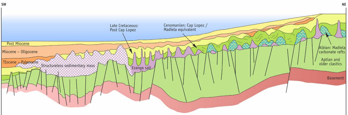
Schematic section through the South Gabon Basin.
